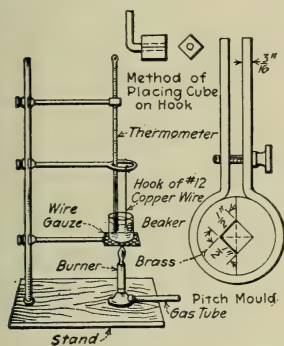
FIG. 178.—Cube Fusing-point Tester.
